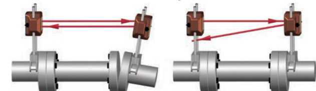
Dual-Beam™ Technology (2 lasers, 1 direction)
